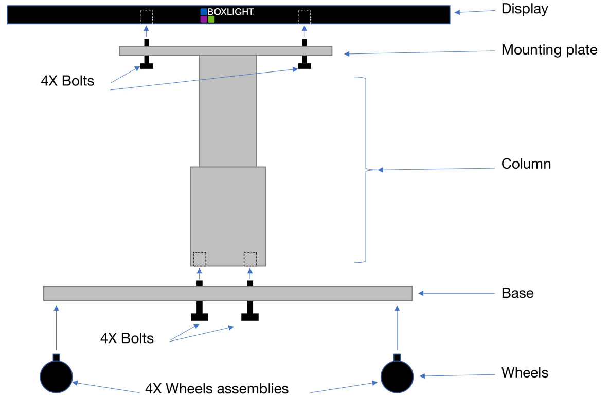
Side View of Base
