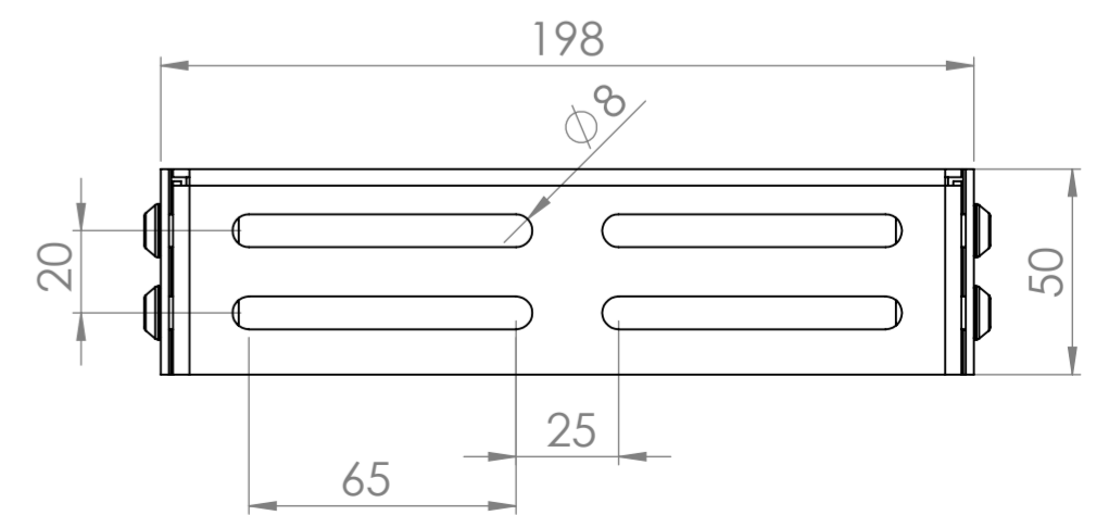
Mount bracket hole pattern
